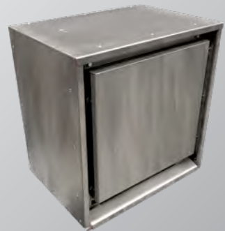
50-3884 C/G Series IPI Power Vent Kit w/110ft Wiring (requires 50-2321 Vent Reducer & 50-4161 Module)
